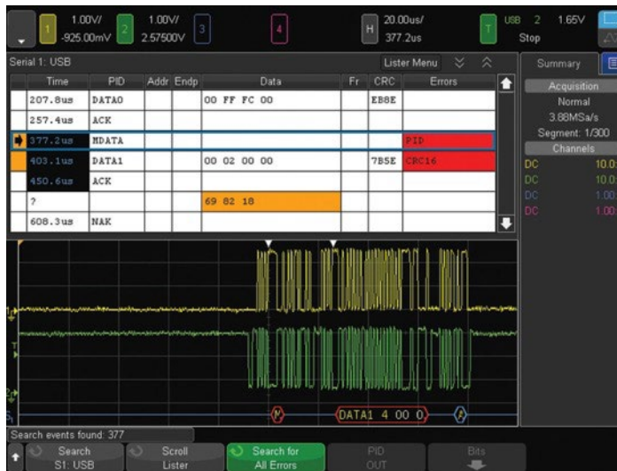
Figure 21. USB 2.0 trigger, decode and “lister” display.
